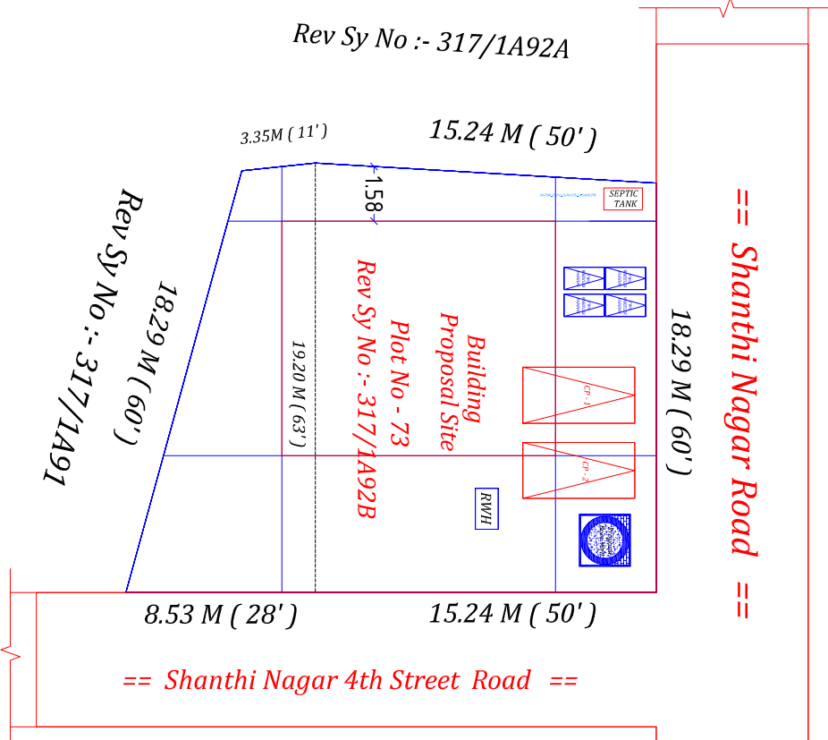
Site Plan - (Scale 1:250)
