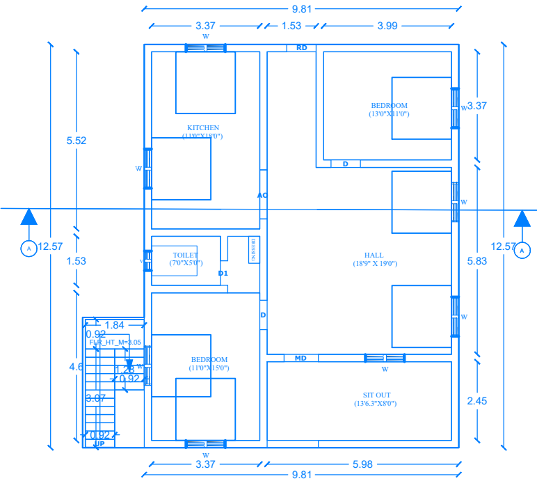
R PLAN
