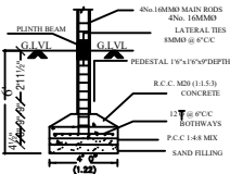
FOUNDATION DETAIL
