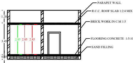
SECTION XX-YY
