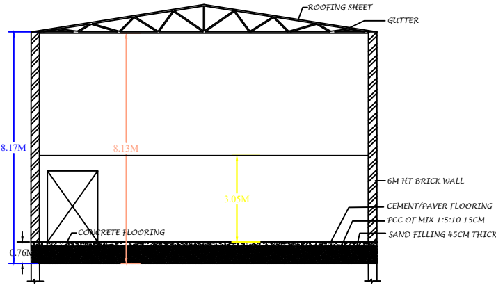
CROSS SECTION ON XX
