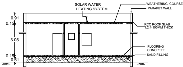
SECTION NP
