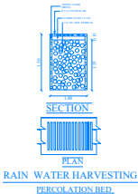
RAIN WATER HARVESTING PERCOLATION BED
