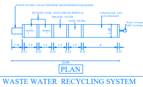
WASTE WATER RECYCLING SYSTEM
