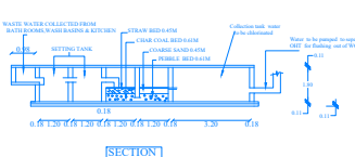
RAIN WATER HARVESTING PERCOLATION PIT
