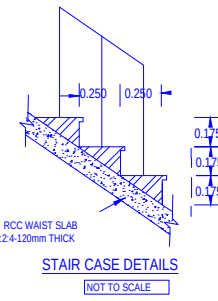
STAIR CASE DETAILS SCALE 1:50
