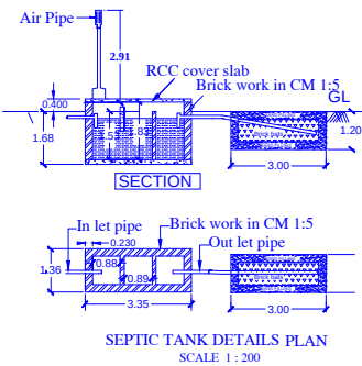
SEPTIC TANK DETAILS PLAN SCALE 1:200
