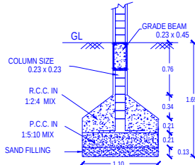
COLUMN DETAILS SCALE 1:50
