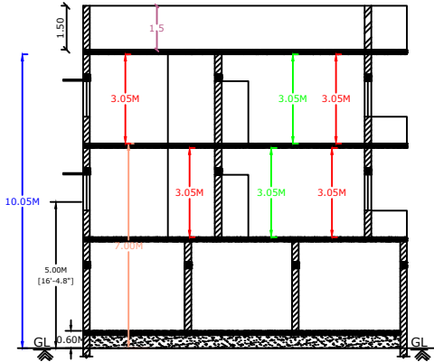
SECTION ON XX
