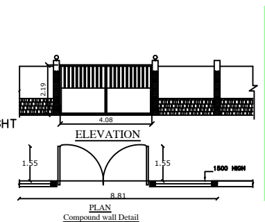
PLAN Compound wall Detail
