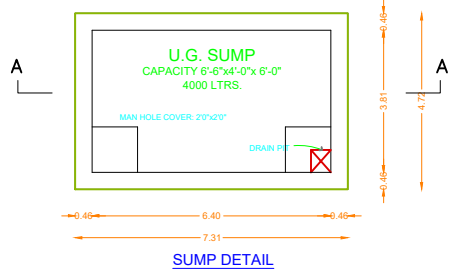
SUMP DETAIL SCALE 1"=4"
