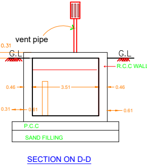
SECTION ON D-D
