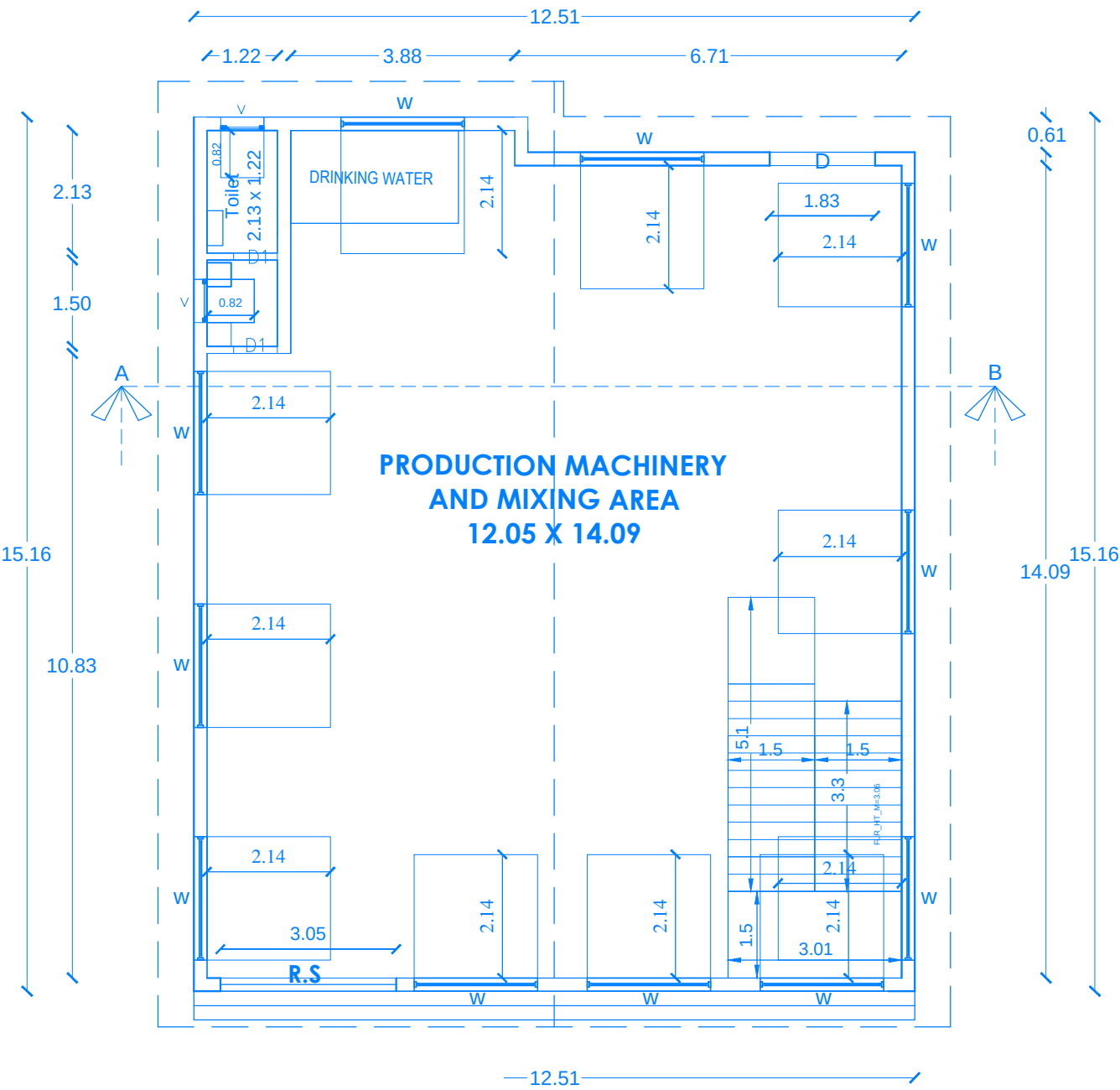
FLOOR PLAN
