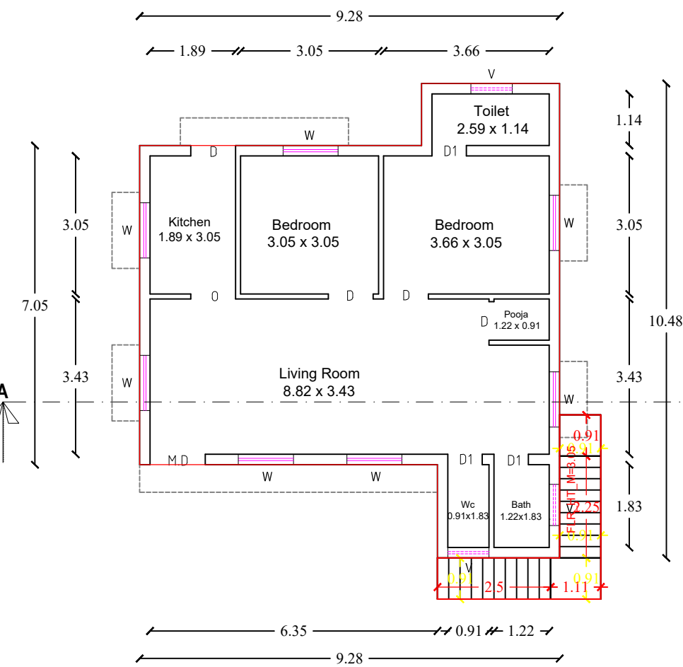
EXI-GROUND FLOOR PLAN
