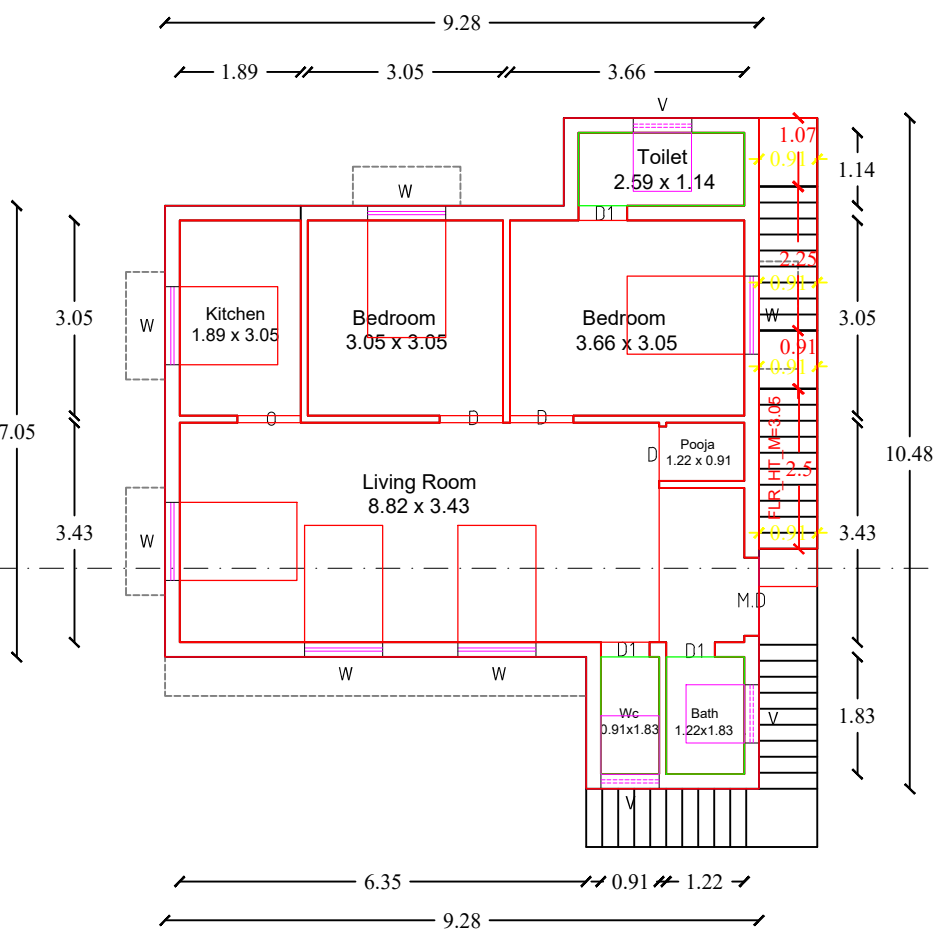
PRO-FIRST FLOOR PLAN
