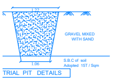
TRIAL PIT DETAILS
