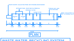
WASTE WATER RECYCLING SYSTEM
