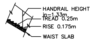
STAIRCASE DETAILS
