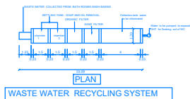
WASTE WATER RECYCLING SYSTEM
