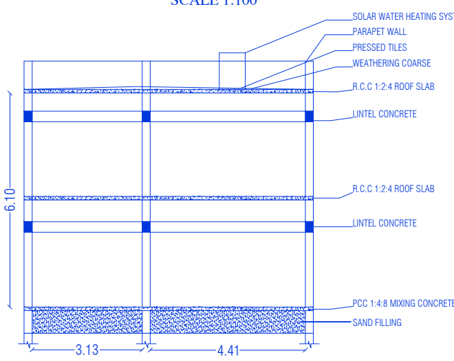
SECTION 8.23 'A-A'
