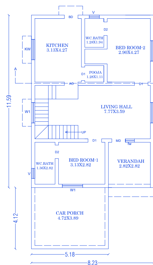
PRO-GROUND FLOOR
