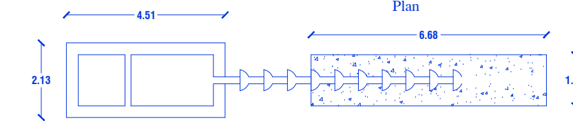
PLAN OF SEPTIC TANK SCALE 1:100
