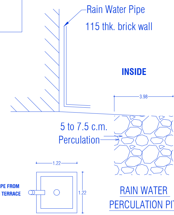
3.RAIN WATER COLLECTION SYSTEM FROM TERRACE
