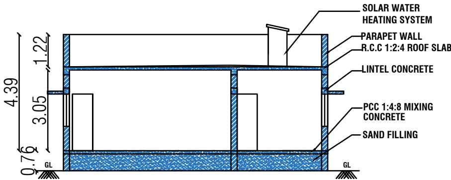
SECTION NO - "AB"
