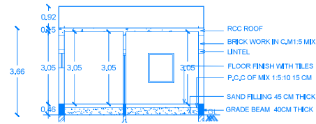
SECTION-AB
