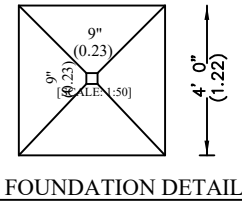
FOUNDATION DETAIL
