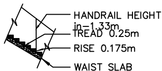
STAIRCASE DETAILS
