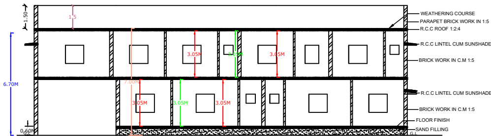
SECTION ON XX
