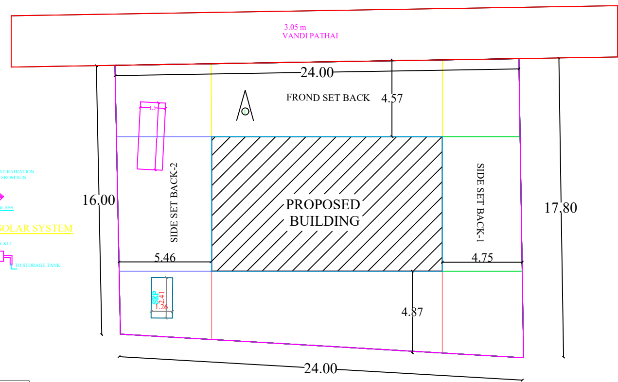
SITE PLAN
