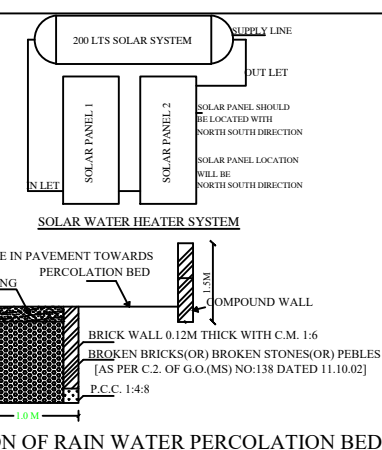
SECTION OF RAIN WATER PERCOLATION BED
