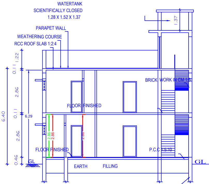
SECTION "A-B"
