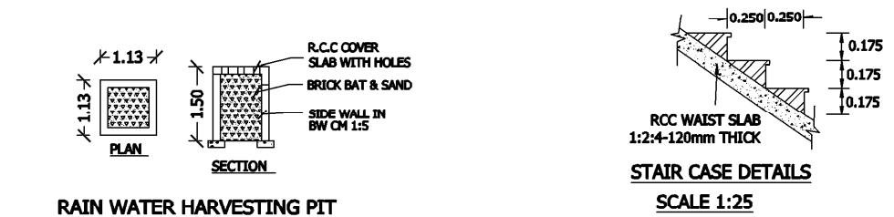
RAIN WATER HARVESTING PIT
