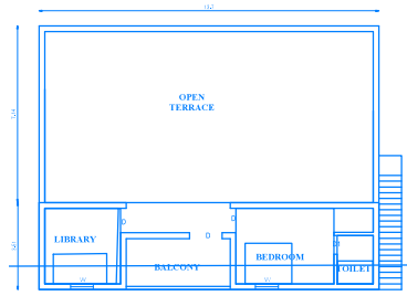
PRO-FIRST FLOOR PLAN
