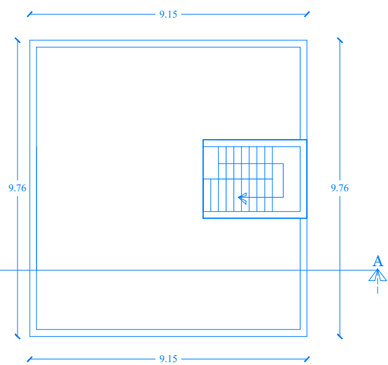
TERACE FLOOR PLAN
