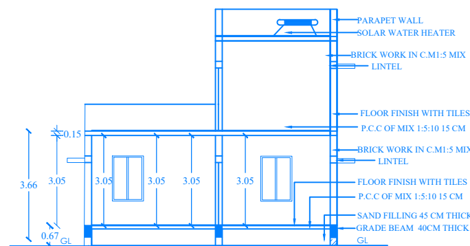
SECTION ON A-A1
