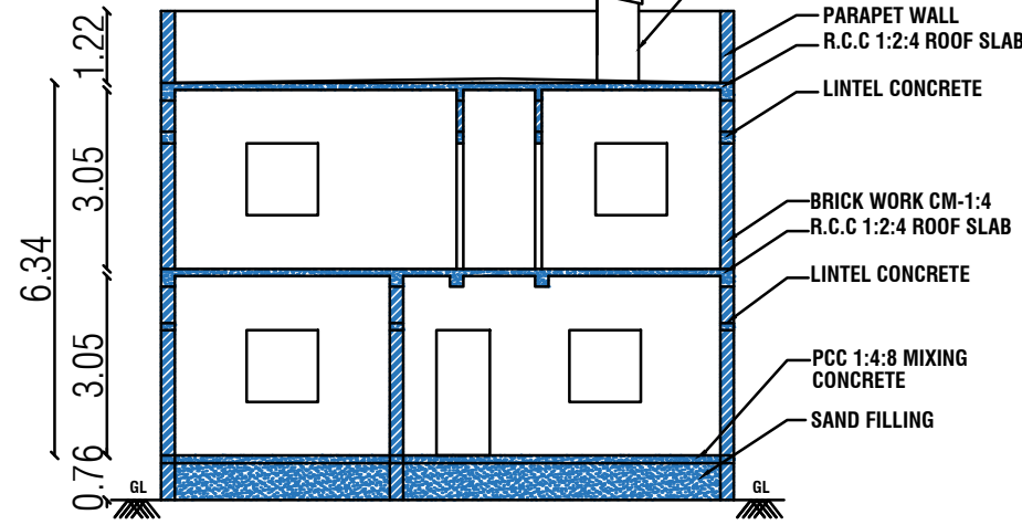
SECTION NO -"AB"
