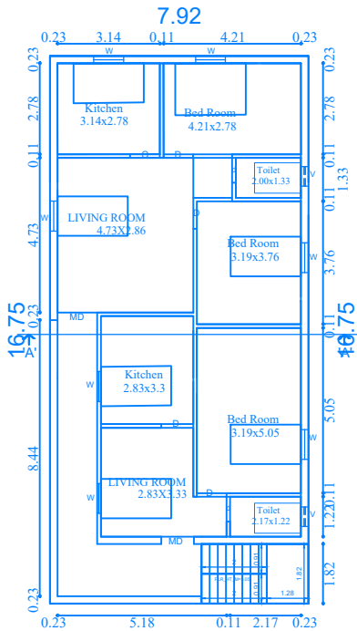
7.92 PRO-FIRST FLOOR PLAN
