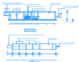
COMPOUND GATE
