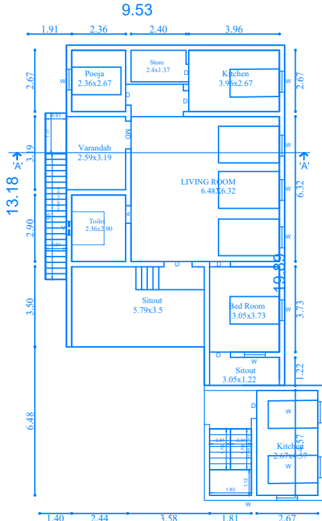
9.53 PRO.FIRST FLOOR PLAN
