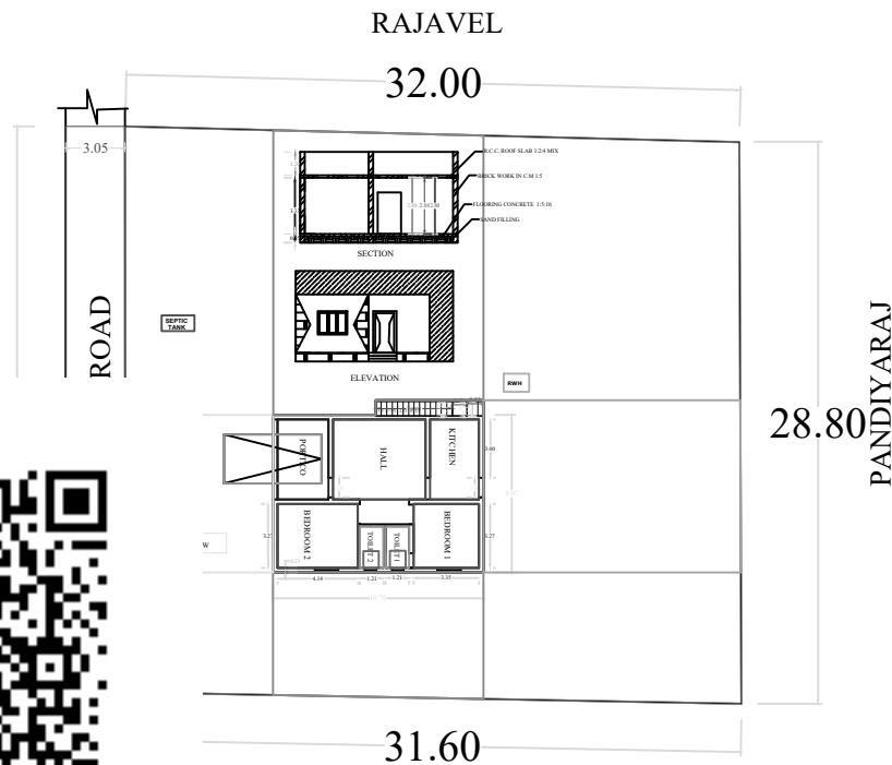
SATHYASEELAN GROUND FLOOR PLAN & SITE PLAN
