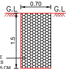
SECTION OF PEBBLE TRENCH
