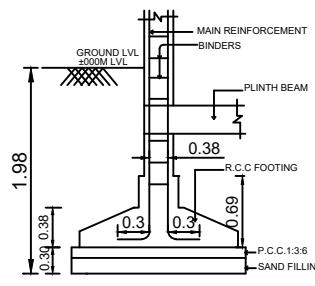
TYPICAL SECTION OF R.C.C FOUNDATION
