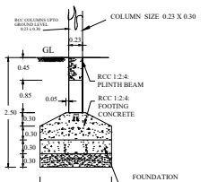
FOUNDATION DETAILS
