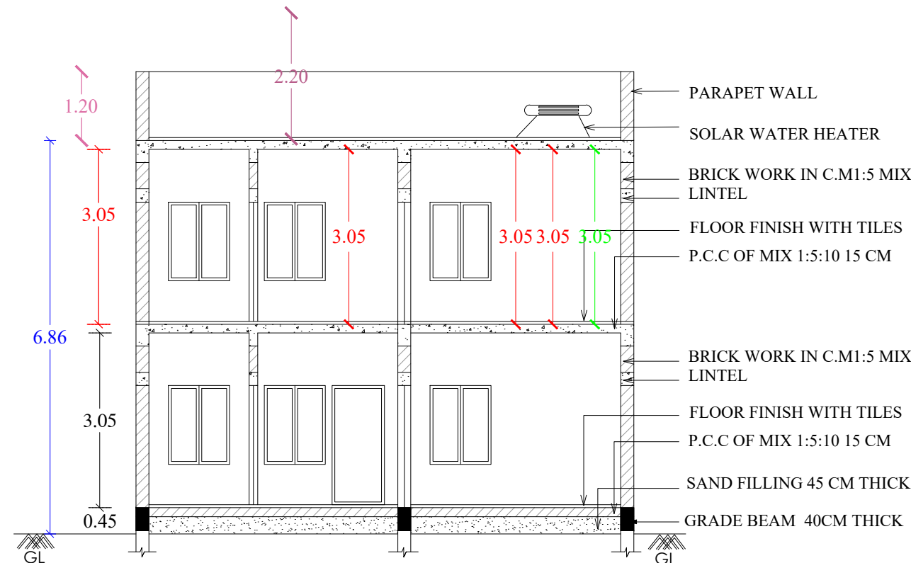
SECTION- AA1
