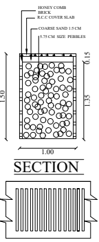
RAIN WATER HARVESTING PERCOLATION BED
