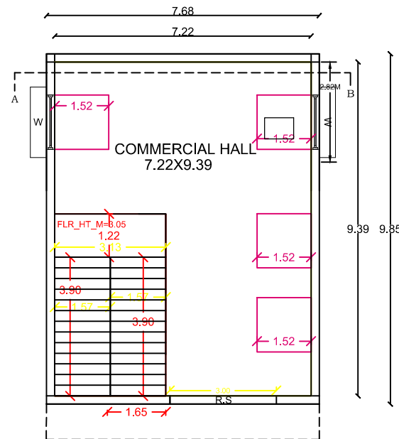
PRO. FIRST FLOOR
