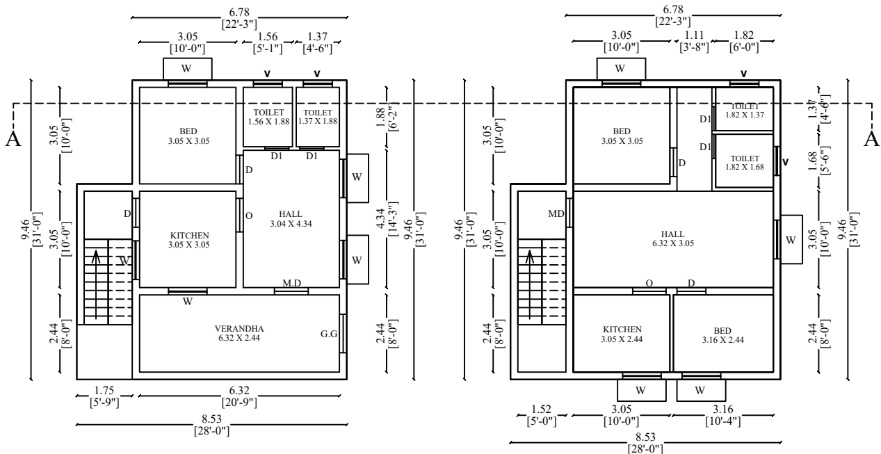
TYPICAL_FLOOR_PLAN=1,2
