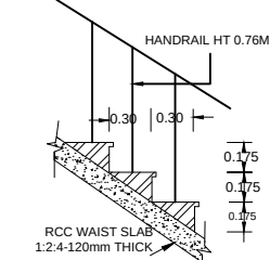
STAIR CASE STEPS SCALE 1:25
