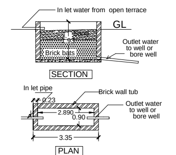
RAIN WATER HARVESTING TANK NOT TO SCALE
