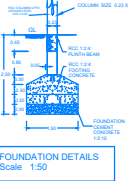
FOUNDATION DETAILS Scale: 1:50
