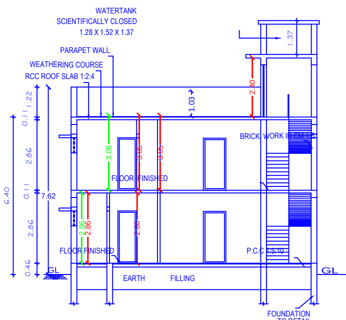
SECTION X-Y
