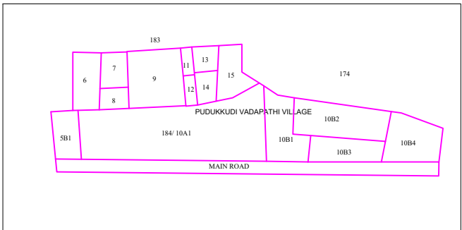
TOPO PLAN
