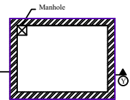
Sump Detail - Plan Capacity - 1000 lt
