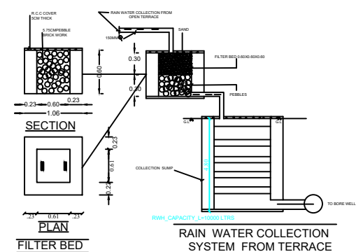
FILTER BED
