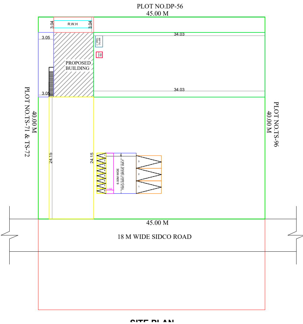
SITE PLAN
