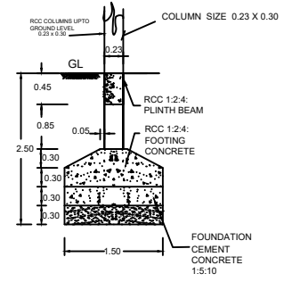
FOUNDATION DETAILS
