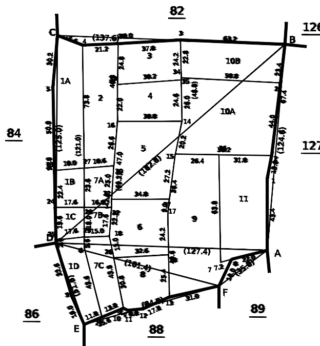
TOPO PLAN
