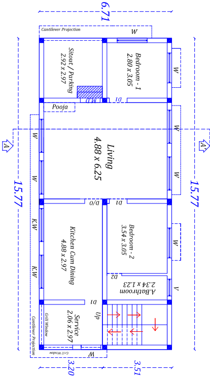
Proposal Ground Floor Plan (Site Plan is in West Facing)
