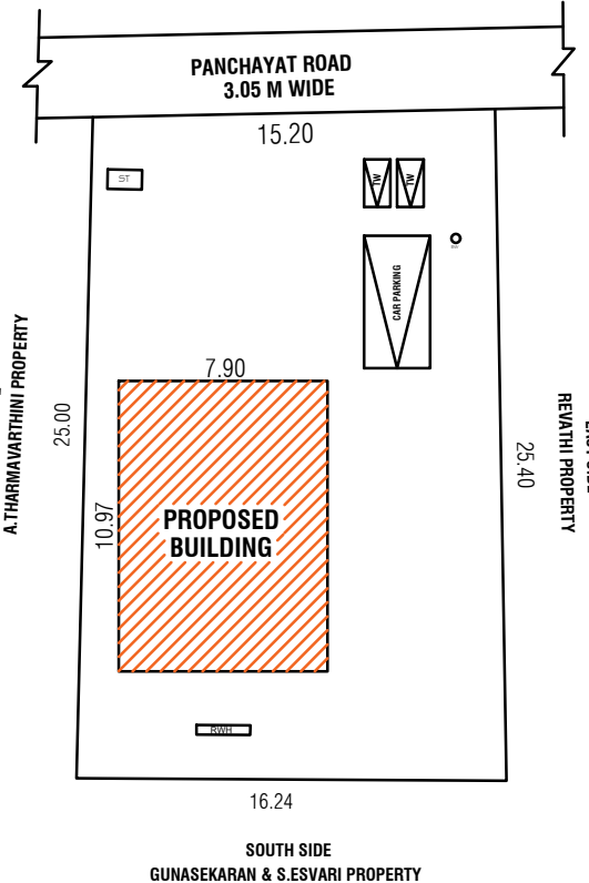
LOCATION PLAN NTS
