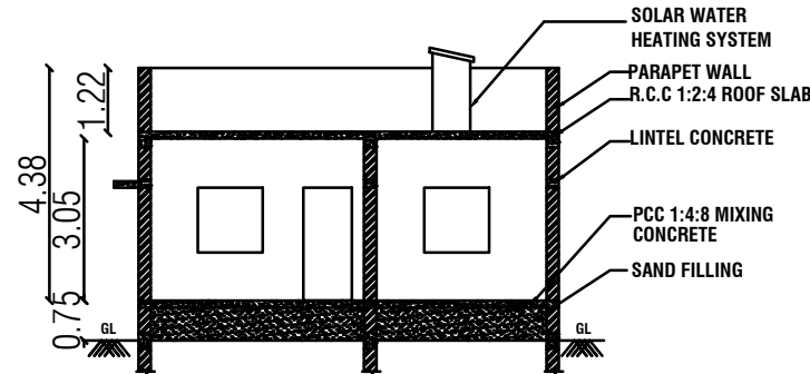
SECTION NO - "AB"
