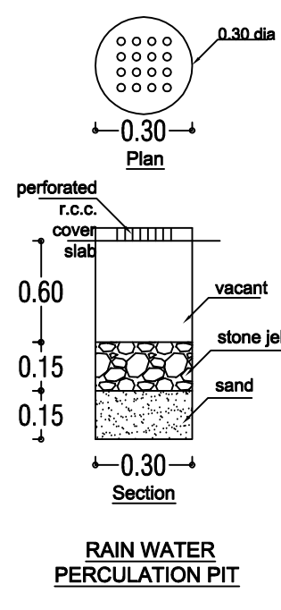
RAIN WATER PERCOLATION PIT
