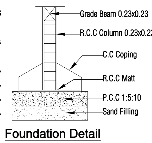
Foundation Detail
