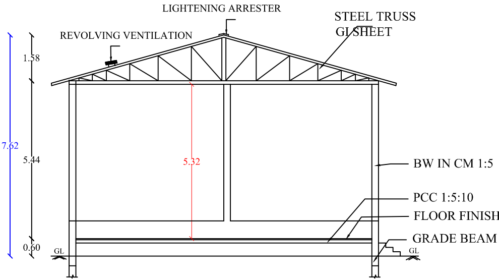
SECTION - XX
