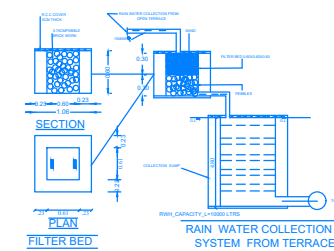
RAIN WATER COLLECTION SYSTEM FROM TERRACE
