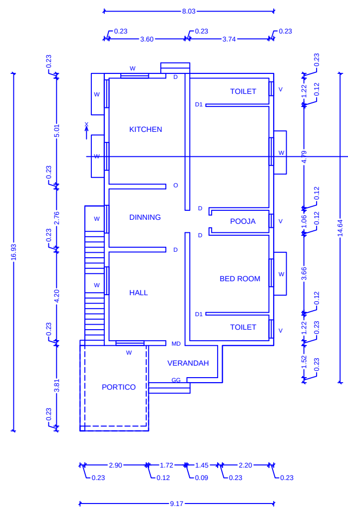
EXIG - GROUND FLOOR PLAN
