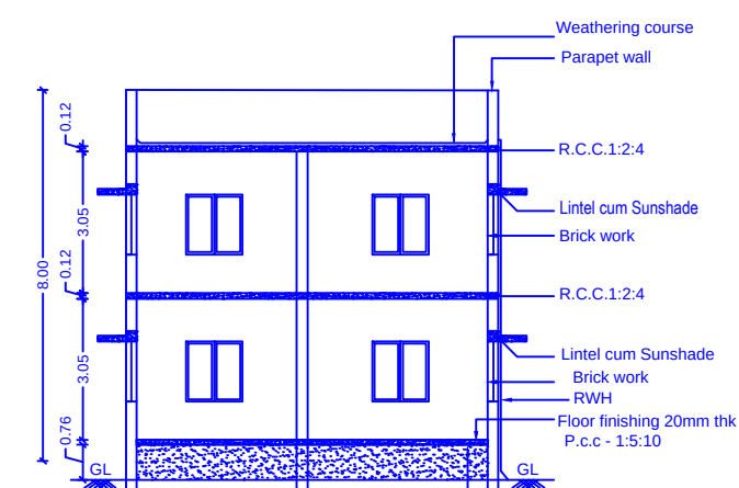
SECTION X-Y
