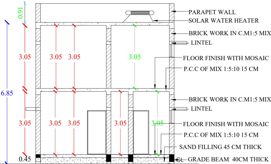
SECTION- AB
