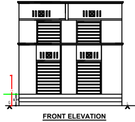
FRONT ELEVATION
