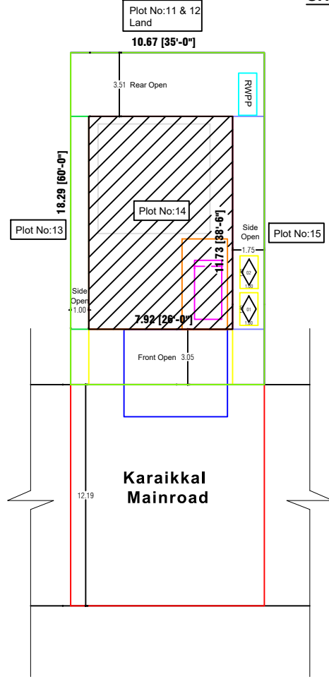
SITE PLAN
