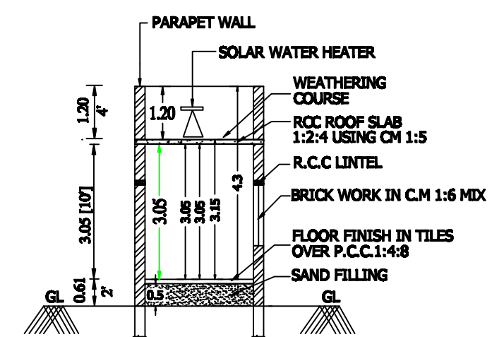
SECTION ON XX'
